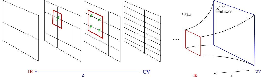
Figure 11: The extra (‘radial’) dimension of the bulk is the resolution scale of the field theory. The left figure indicates a series of block spin transformations labelled by a parameter z . The right figure is a cartoon of AdS space, which organizes the field theory information in the same way. In this sense, the bulk picture is a hologram: excitations with different wavelengths get put in different places in the bulk image.
